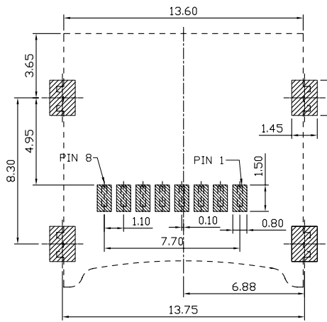
RECOMMENDED PCB LAYOUT TOLERANCES: ±0.05
