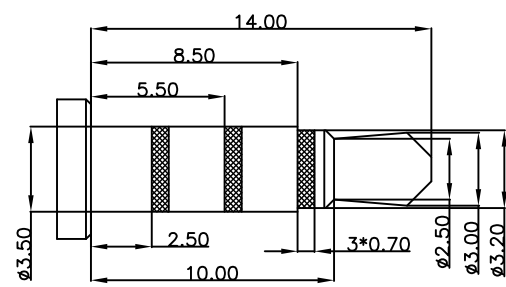
\phi 3.50 mm 4 POLE PLUG
