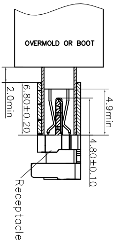
Mated Condition
